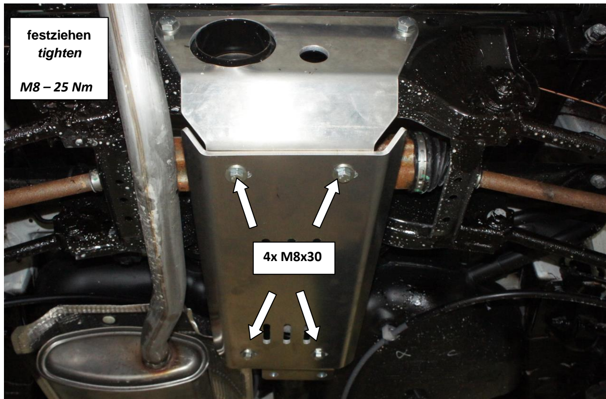
Schutzplatte "A" anbringen / Attach skid plate "A"
