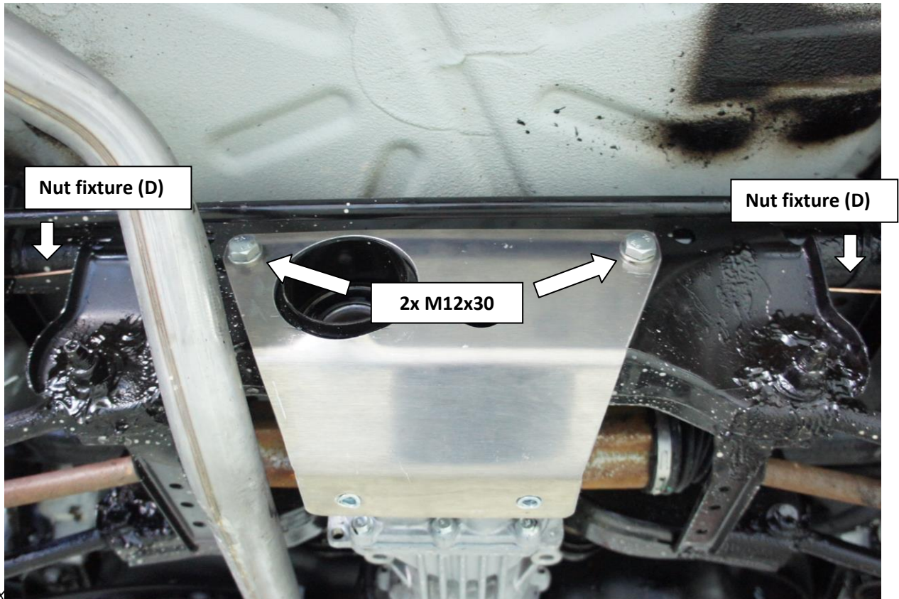
Konsole "C" anbringen / Attach bracket "C"
