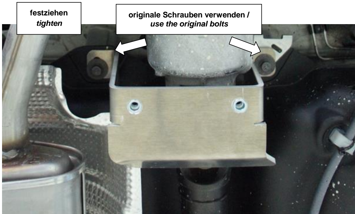
Konsole "B" anbringen / Attach bracket "B"
